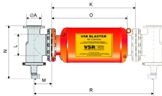
VSR BLASTER® Air cannon Type EV1 and EV2, with external valve
