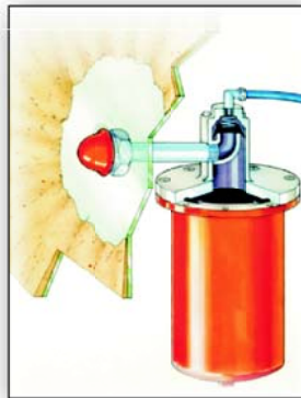
ERPULSOR® air injector
