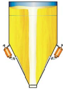
Ratholing
